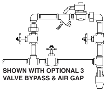
FIGURE B Three-valve Make-up Bypass
