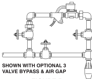
FIGURE B Three-valve Make-up Bypass
